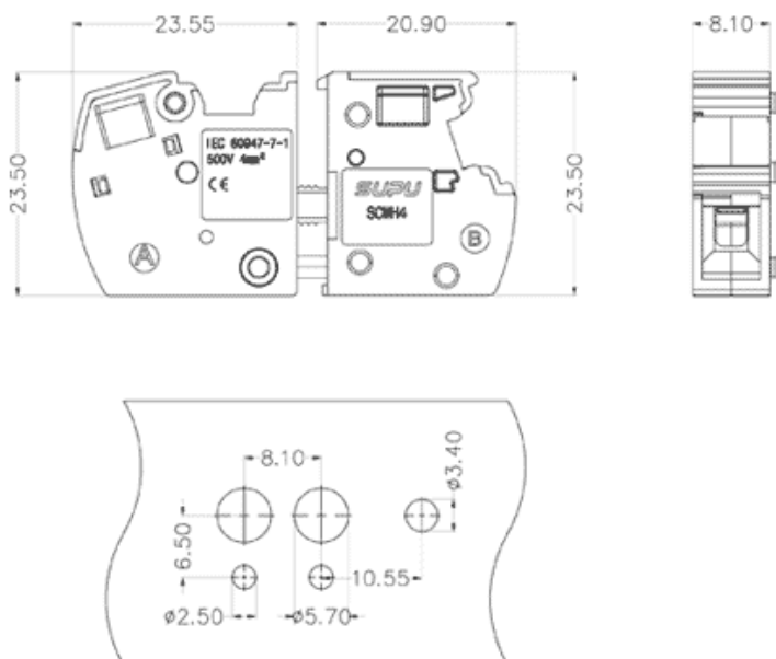
钻孔图 For a drilling diagram
